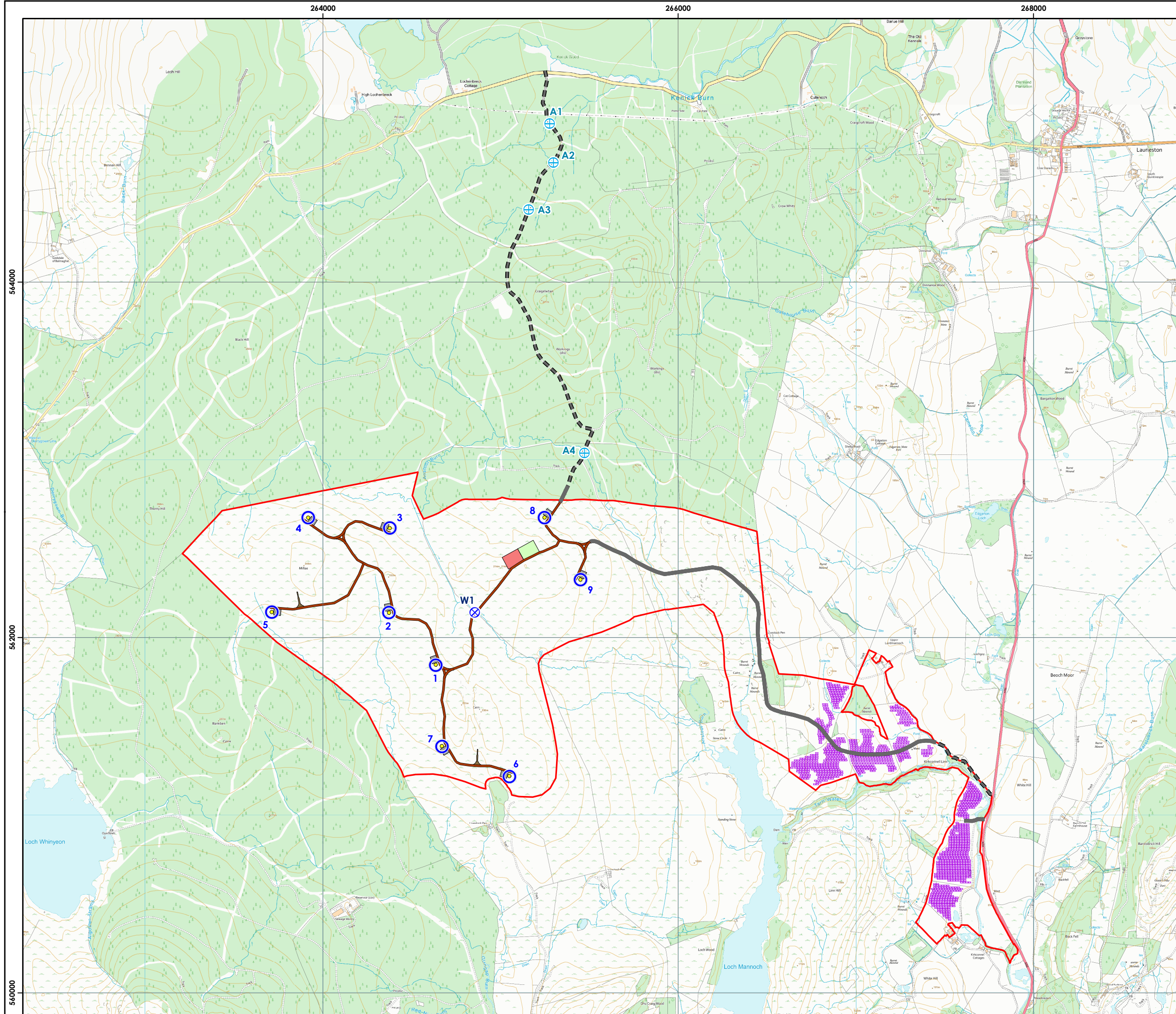
Figure 3 Site Layout
