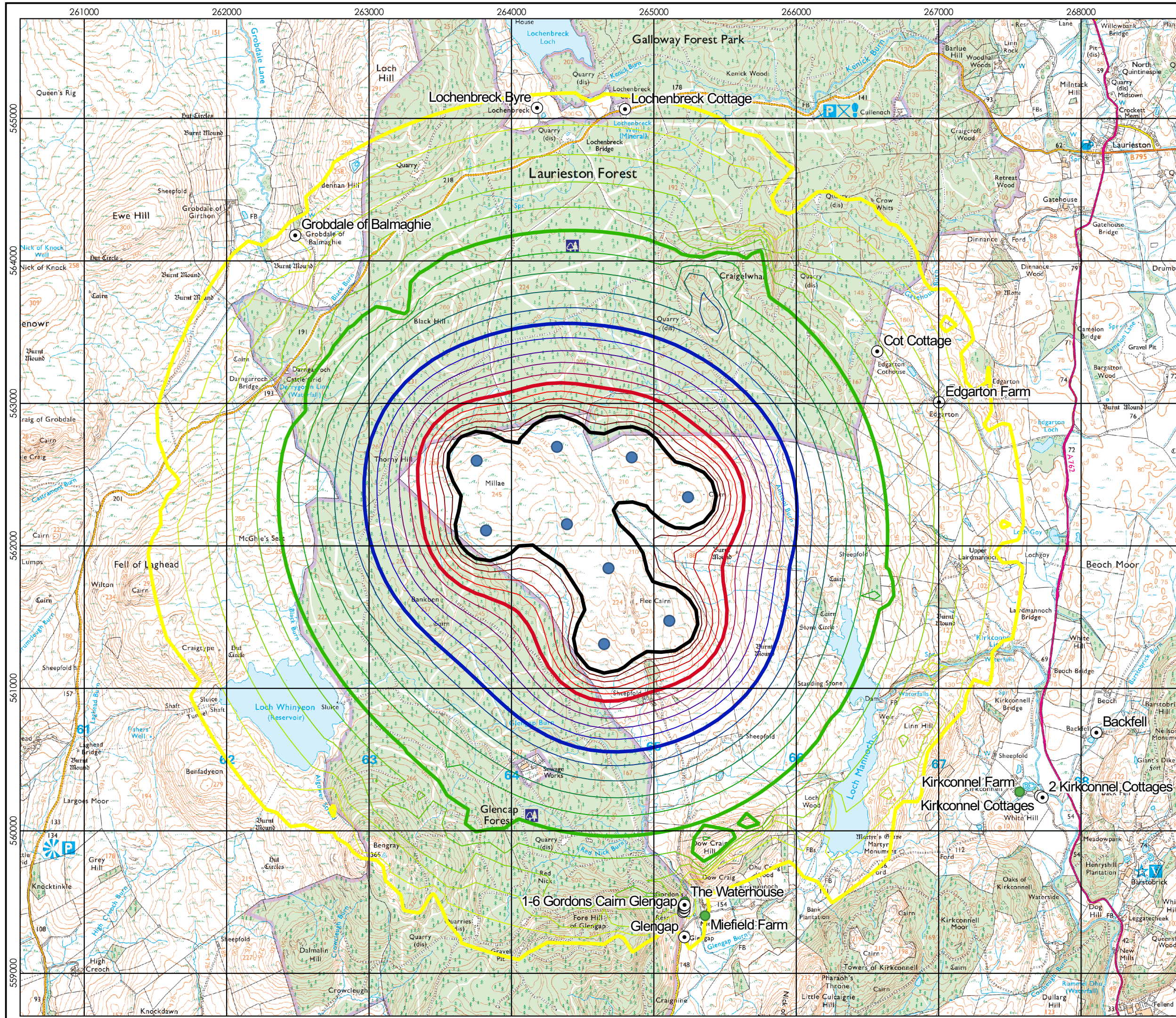
Figure 9-2 Predicted Wind Turbine Operational Noise Contours at 7-12 m/s
