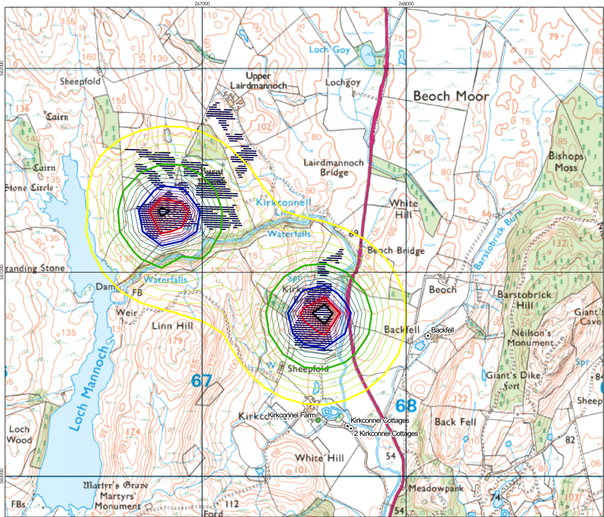
Figure 9-1 Predicted Solar Operational Noise Contours
