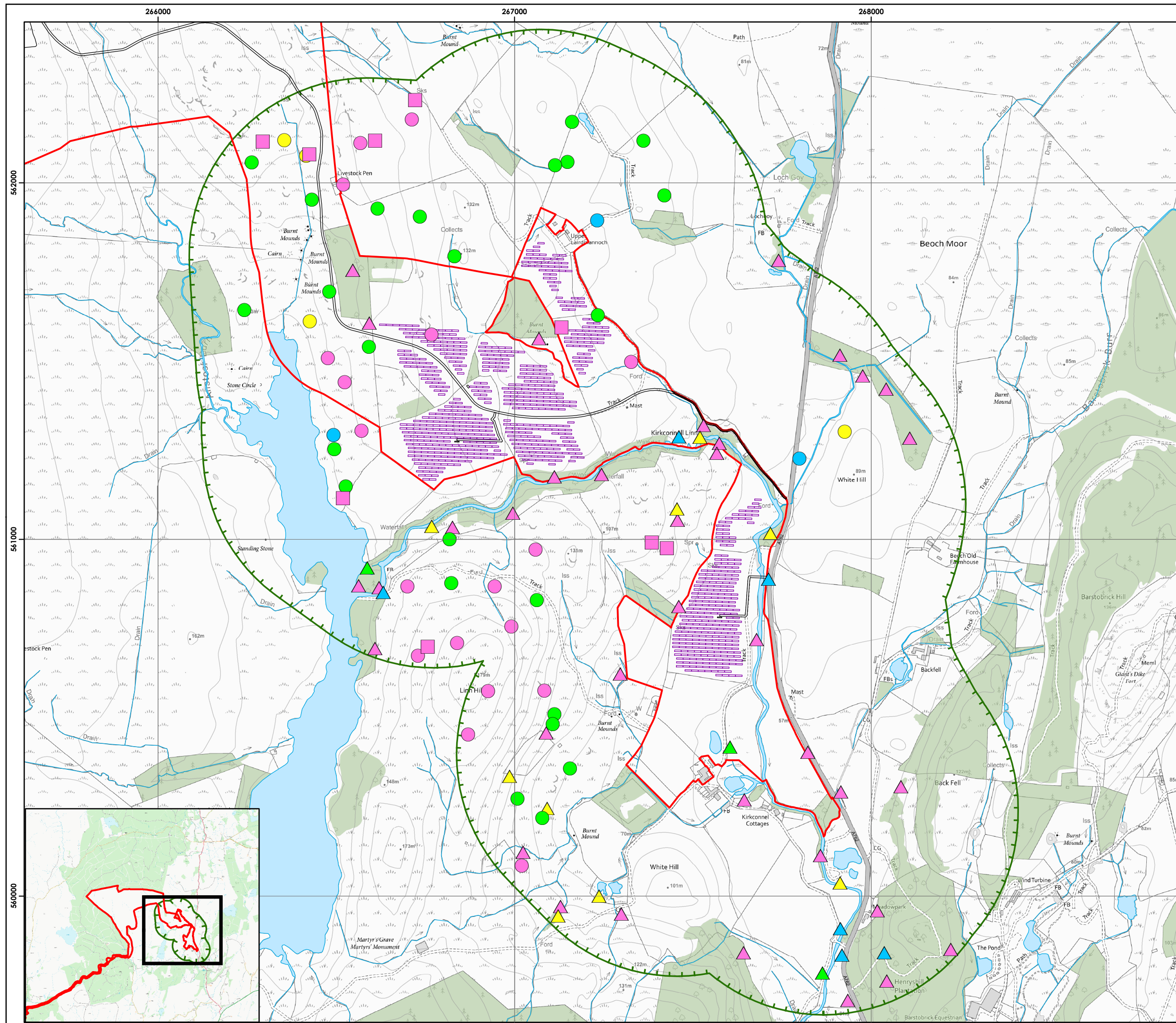
Figure 7-1-8a Breeding Bird Results - 2023 Numerous Species
