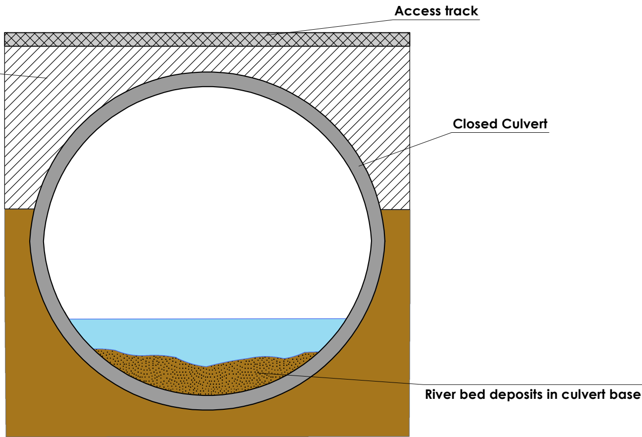
INDICATIVE CLOSED CULVERT
