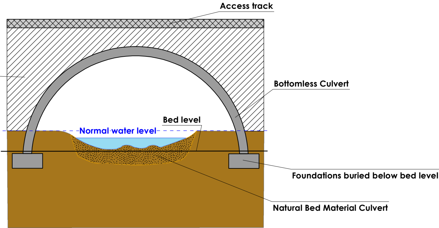
INDICATIVE BOTTOMLESS CULVERT
