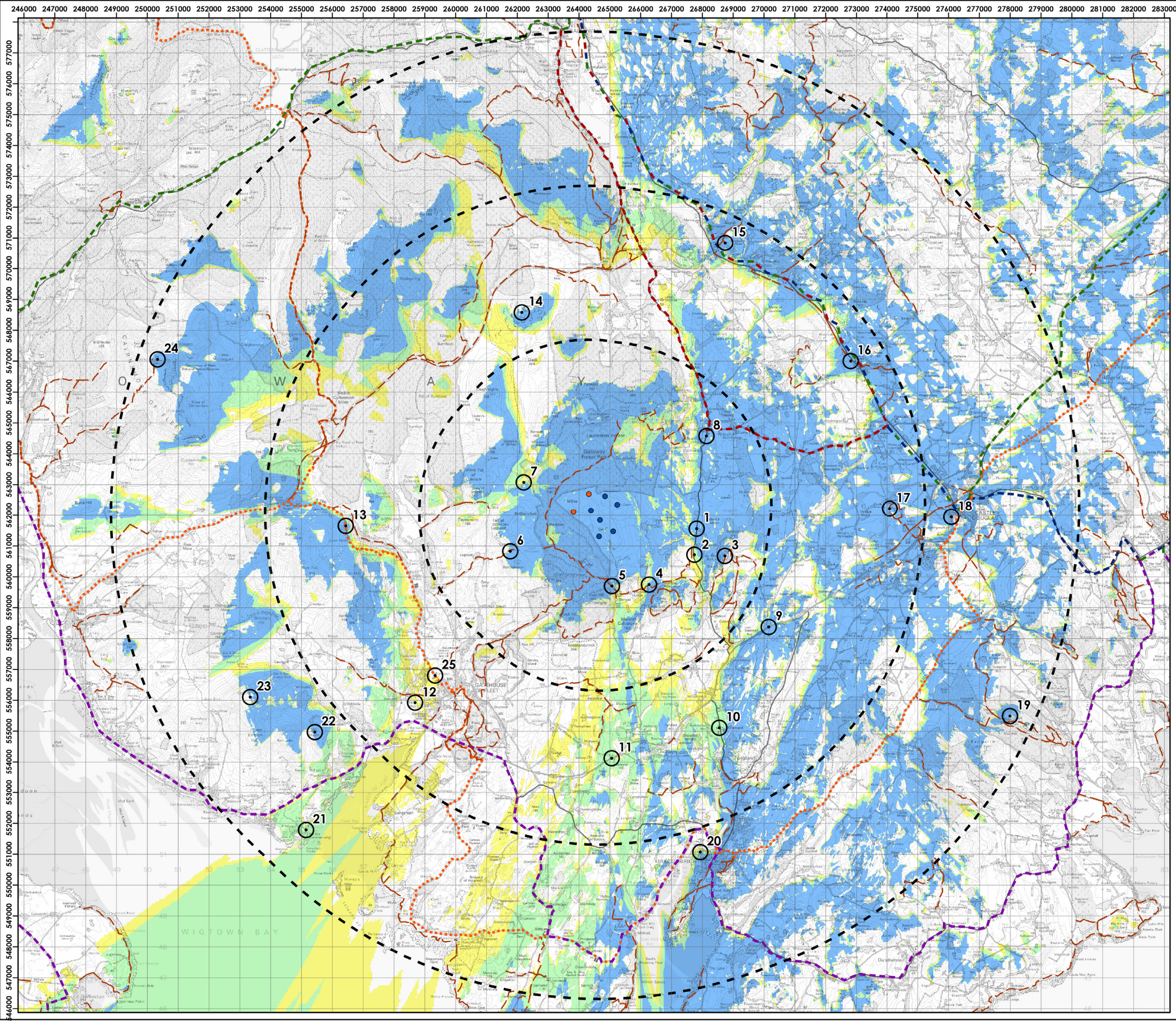
AI Figure 5-6 Visual Receptor Locations with Zone of Theoretical Visibility - Bare Ground
