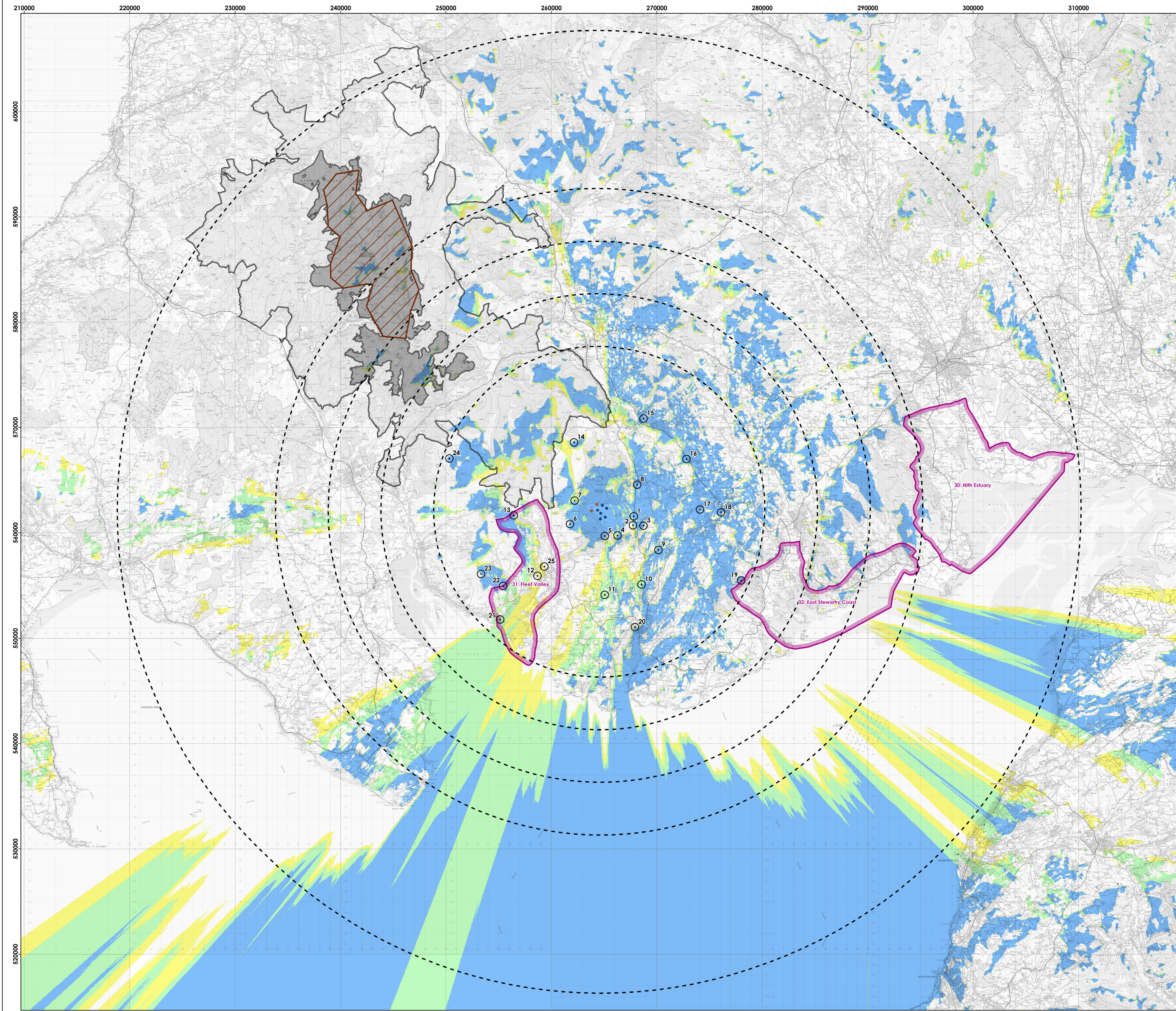
AI Figure 5-3 Zone of Theoretical Visibility to Blade Tip, 45km
