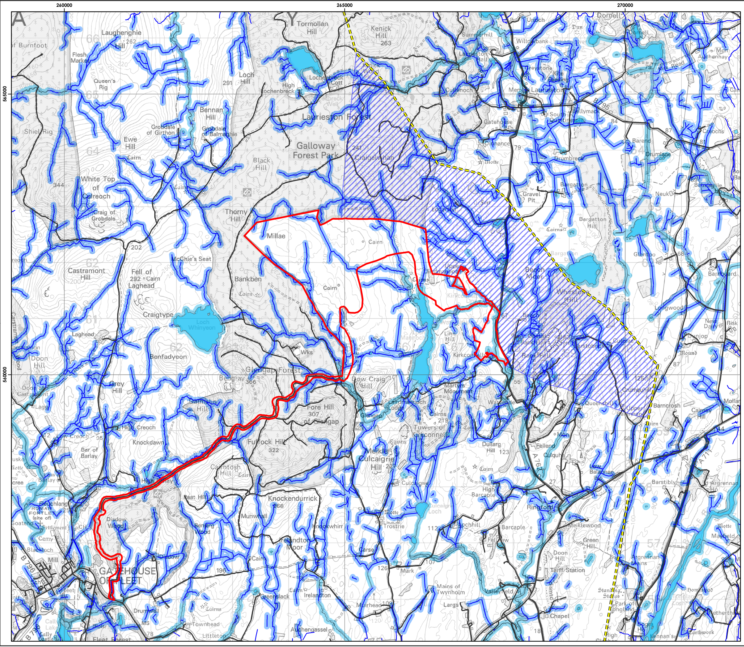
Figure 10 Local hydrology
